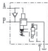
DAW...-50B/...
