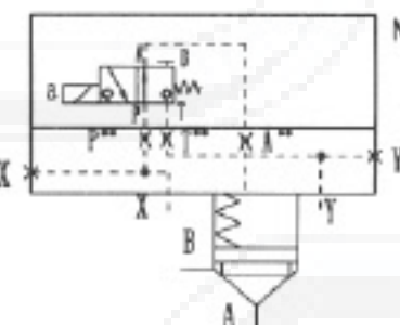
LFA.WEA.6XB/630... Size 80 and 100
