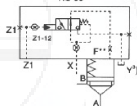
LFA.R2- 6XB/... NS 63
