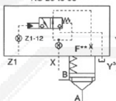
LFA.R2- 6XB/... NS 25 to 50
