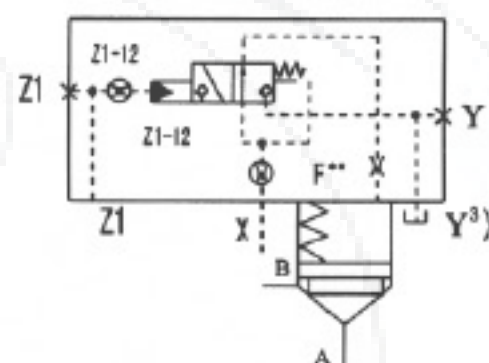
LFA.R2- 6XB/... Size 80 and 100
