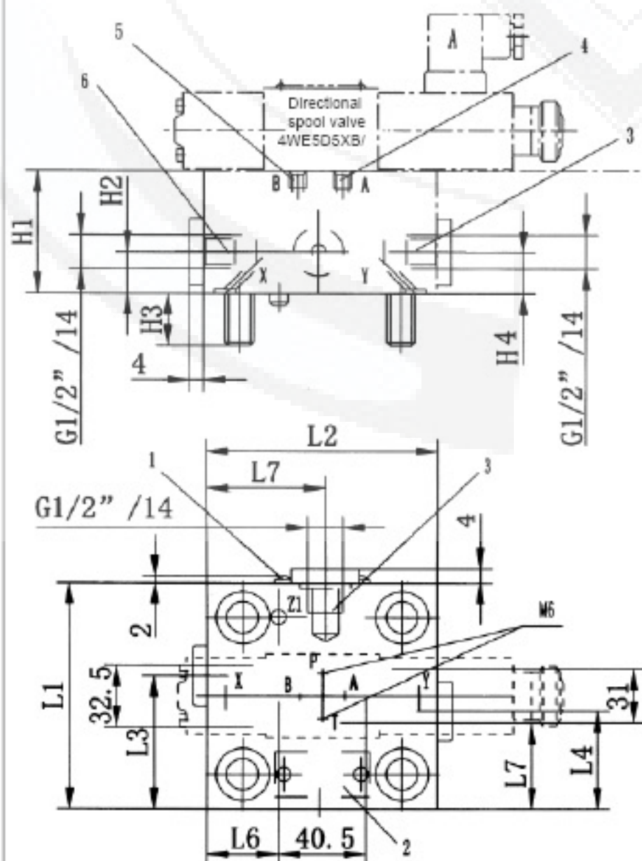
LFA.GWA 6XB/... Size 16 to 32
