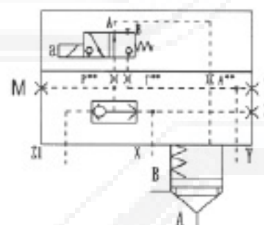
LFA.GWA 6XB/630... Size 80 and 100
