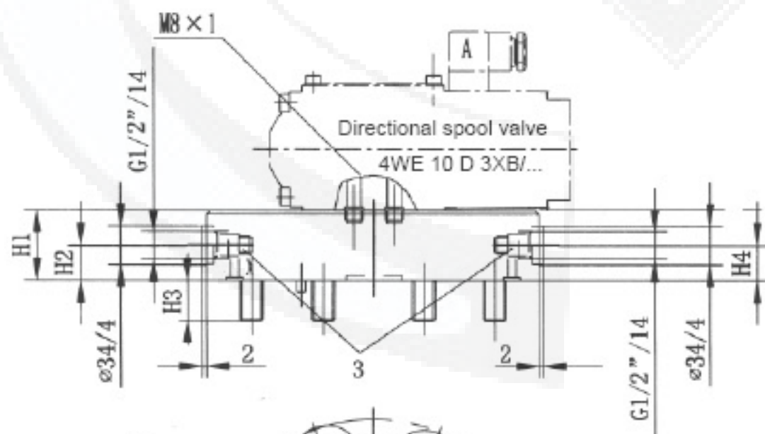
LFA.WEA.6XB/... Size 80 and 100
