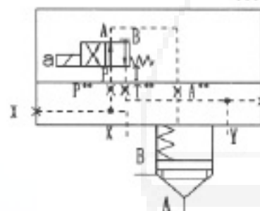
LFA.WEA.6XB/... Size 80 and 100
