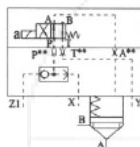
LFA.GWA 6XB/... Size 16 to 32
