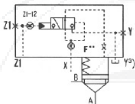
LFA.R 6XB/... Size 80 and 100
