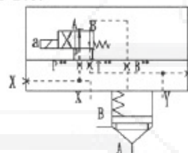
LFA.WEB.6XB/... Size 80 and 100
