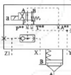
LFA.GWA 6XB/... Size 40 to 63
