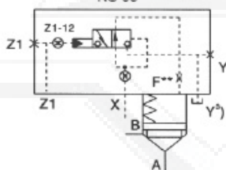
LFA.R 6XB/... NS 63
