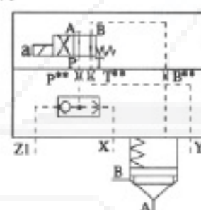
LFA.GWB 6XB/... Size 16 to 32
