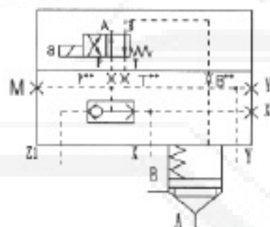
LFA.GWB 6XB/... Size 80 and 100
