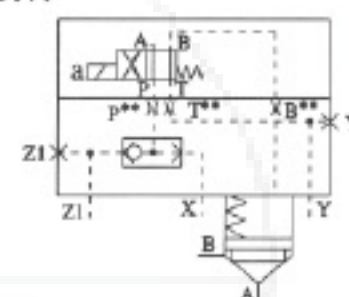
LFA.GWB 6XB/... Size 40 to 63
