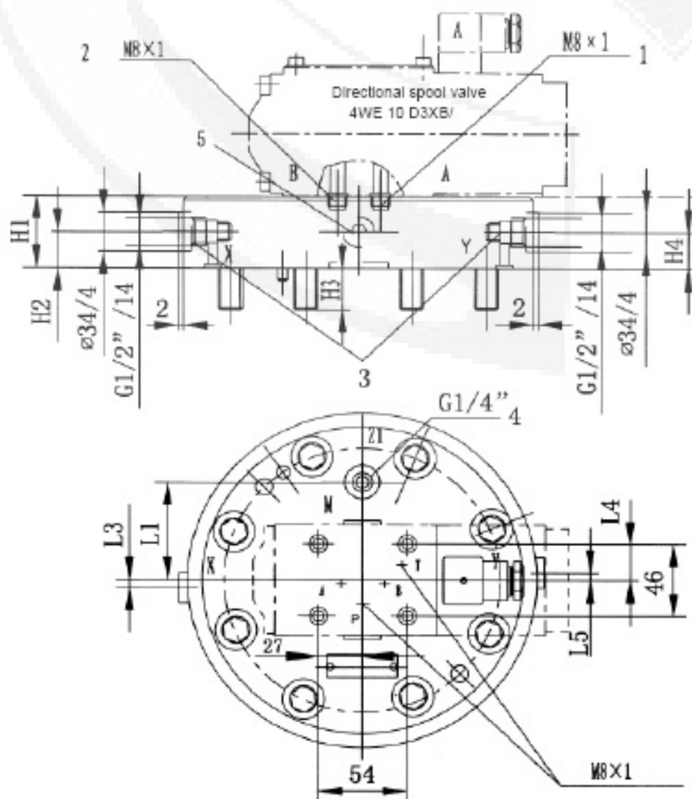
LFA.GWA 6XB/... Size 80 and 100
