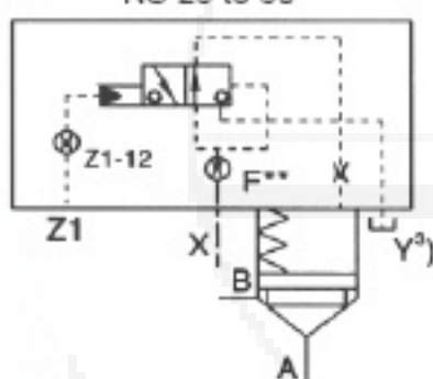
LFA.R 6XB/... NS 25 to 50
