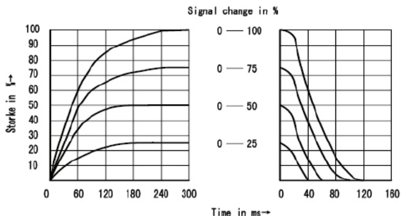
Performance limit, nominal flow 30 L/min
