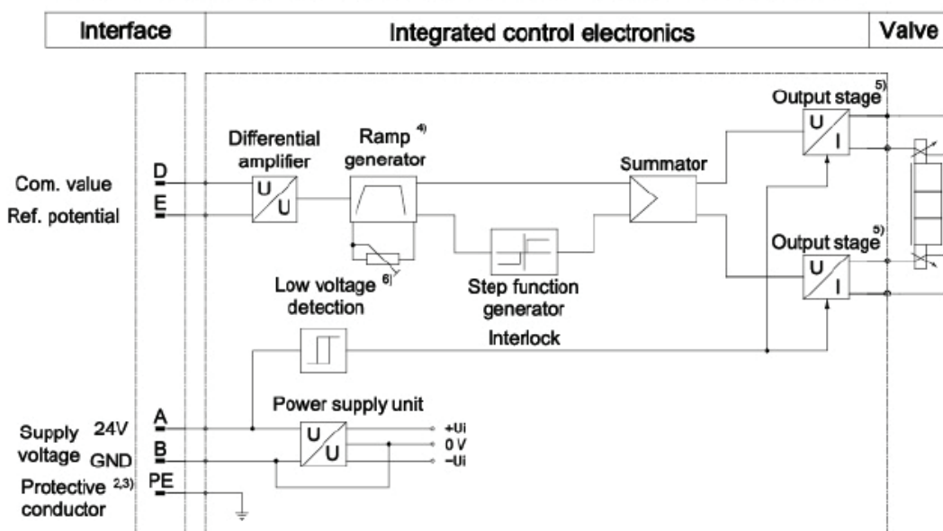
Block circuit diagram/terminal allocation of the integrated control electronics
