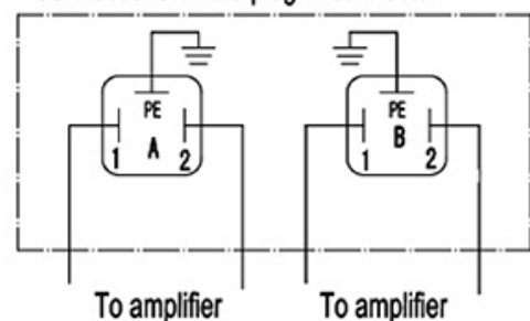
Connections on the plug-in connector
