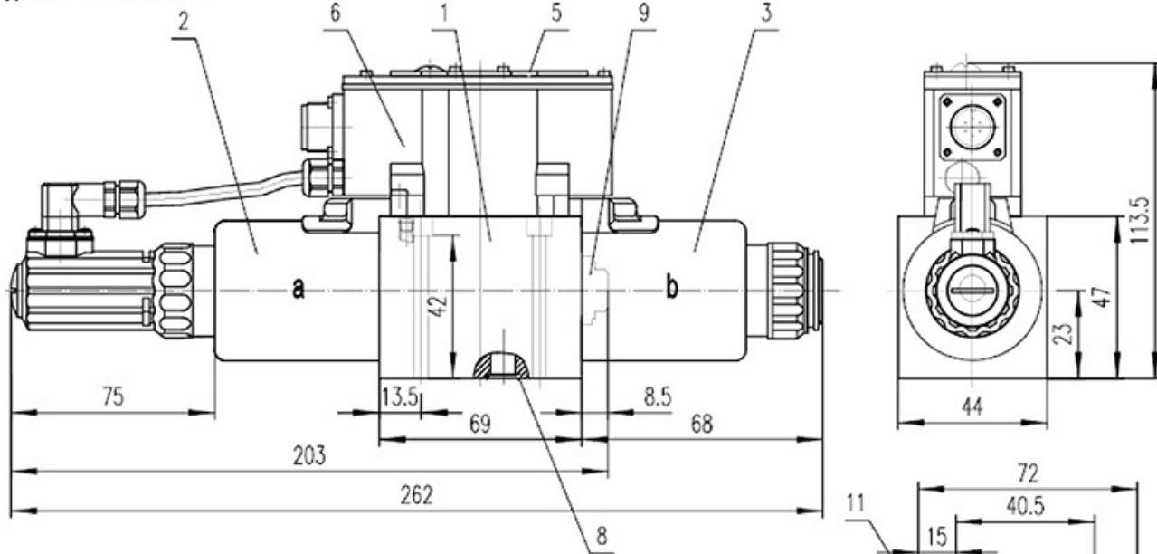
Type HD-4WREE6...-2X/
