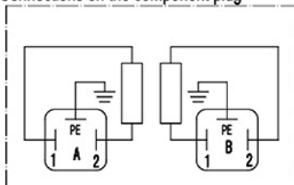
Connections on the component plug
