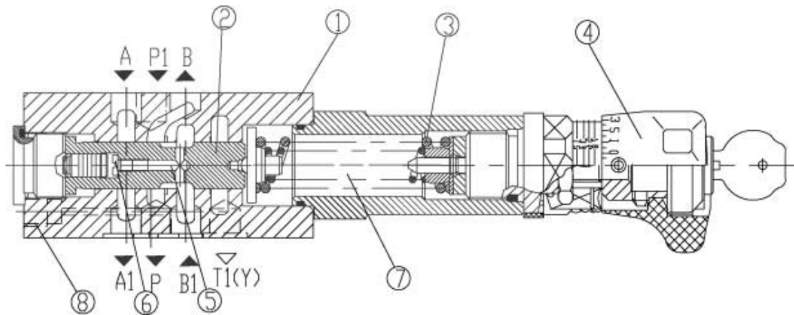
ZDR10D...40B/...YM
